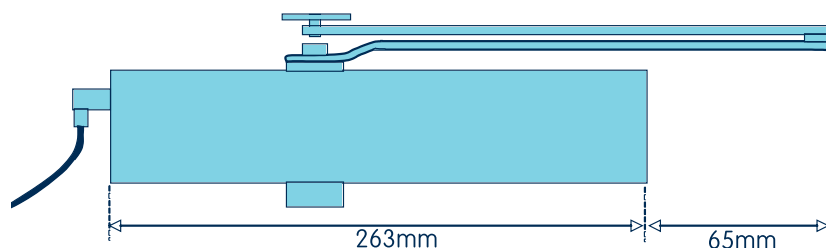
Projecting Arm configuration
